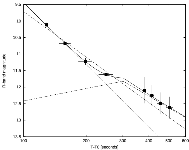
Fig. 3. The R-band afterglow lightcurve of GRB 060117. The lightcurve is fitted as a superposition of reverse shock (dotted line) and forward shock (dashed line). The linear fit is plotted by a dot-and-dash line.
