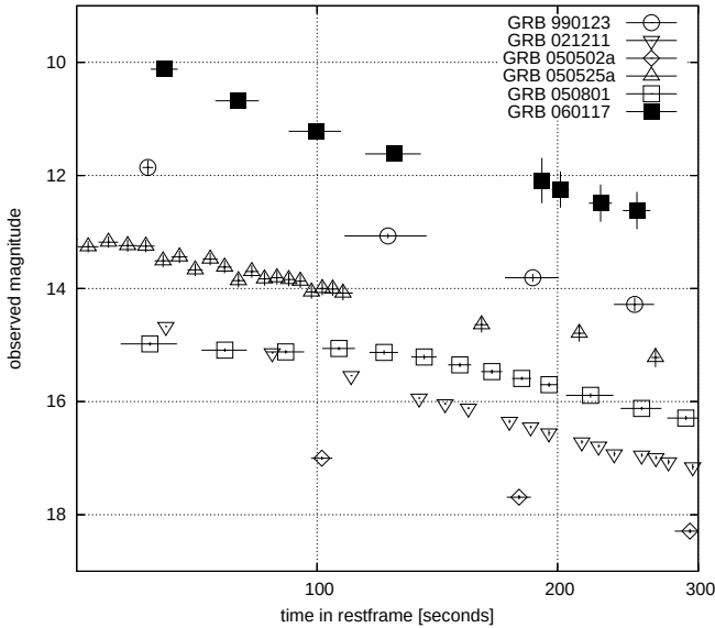
Fig. 1. The optical light curve of GRB 060117 in comparison with other well-covered early GRB optical emissions: GRB 990123 (Akerlof et al., 1999), GRB 021211 (Li et al., 2003), GRB 050502a (Guidorzi et al., 2005), GRB 050525a (Blustin et al., 2006), and GRB 050801 (Rykoff et al., 2006). In this figure we use z \approx 1.0 for GRB 060117. Observed R -band magnitudes are shown, except for GRB 050525a, where the V -band values are plotted.
