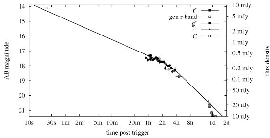
Fig. 2: Overall view of the light curve of GRB080603B
