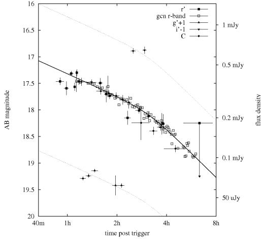
Fig. 1: Detail of the optical light curve of GRB080603B showing the observations by BOOTES (filled symbols) and from the literature (empty symbols)
