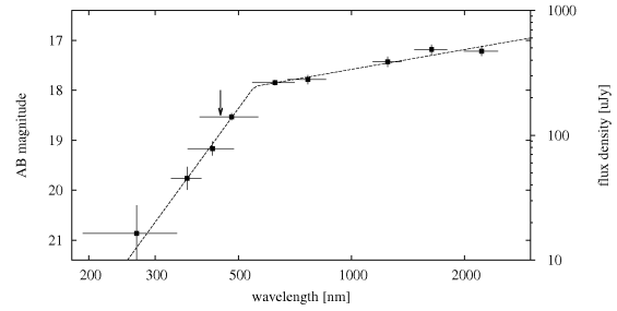
Fig. 4: The spectral energy distribution of the afterglow in rest frame. The small arrow marks Ly- \alpha position for z = 2.69
