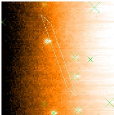
Figure 3. GRB031111A I filter image 25 \times 25 arcmin 2 (0,5% of the WF image)
