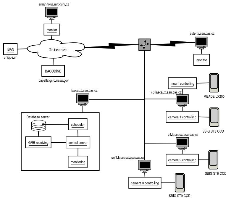
Figure 4. BART - system structure
