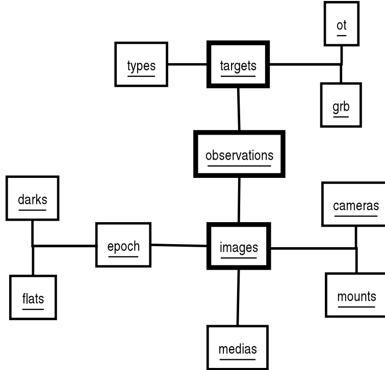
Figure 2. Database structure overview
