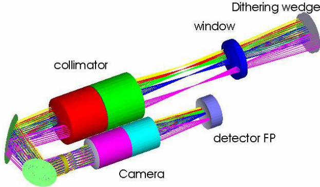
Fig. 2. – The BOOTES-IR camera optical train.
